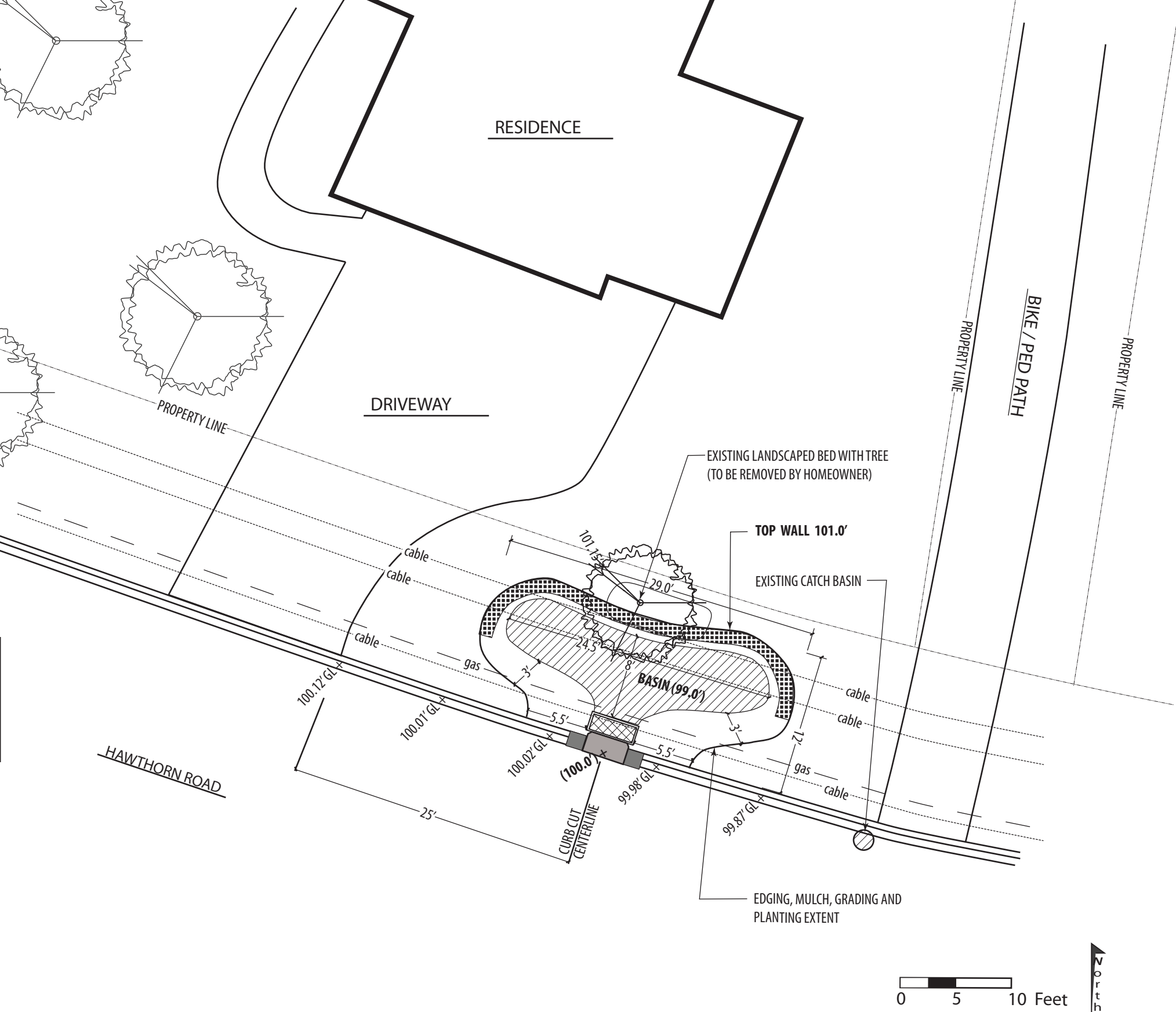
GRADING PLAN (SEE 'SECTION A' ON SHEET 3 FOR TYPICAL RAIN GARDEN WITH WALL)
